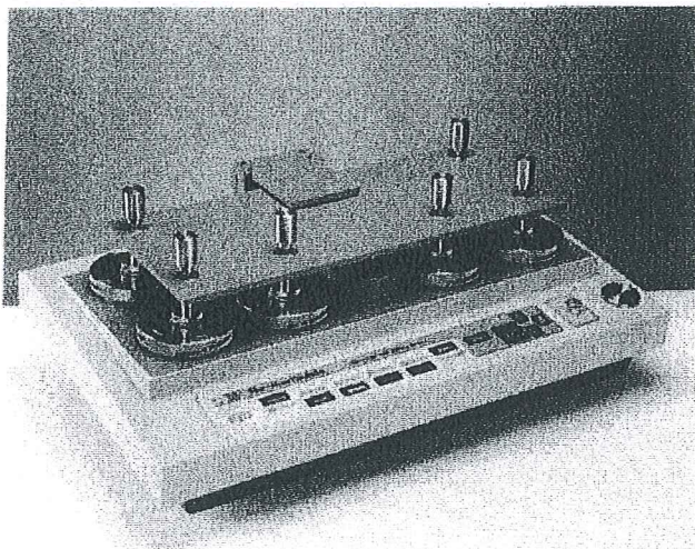
FIG. 1 Martindale Abrasion Tester
