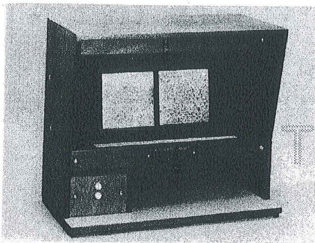
FIG. 2 Apparatus for Fabric Evaluation
